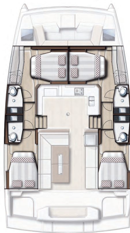
4 CABIN VERSION / 4 BATHS Version 4 cabines / 4 sdb
